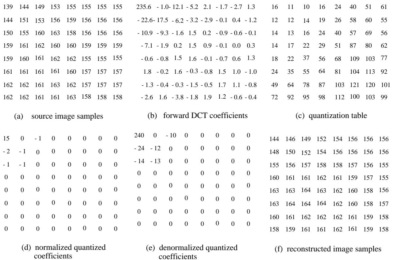
Figure 10. DCT and Quantization Examples
